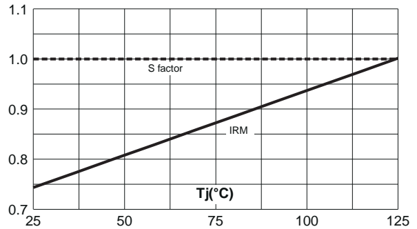
Fig. 7: Relative variation of dynamic parameters versus junction temperature (reference Tj=125°C).
